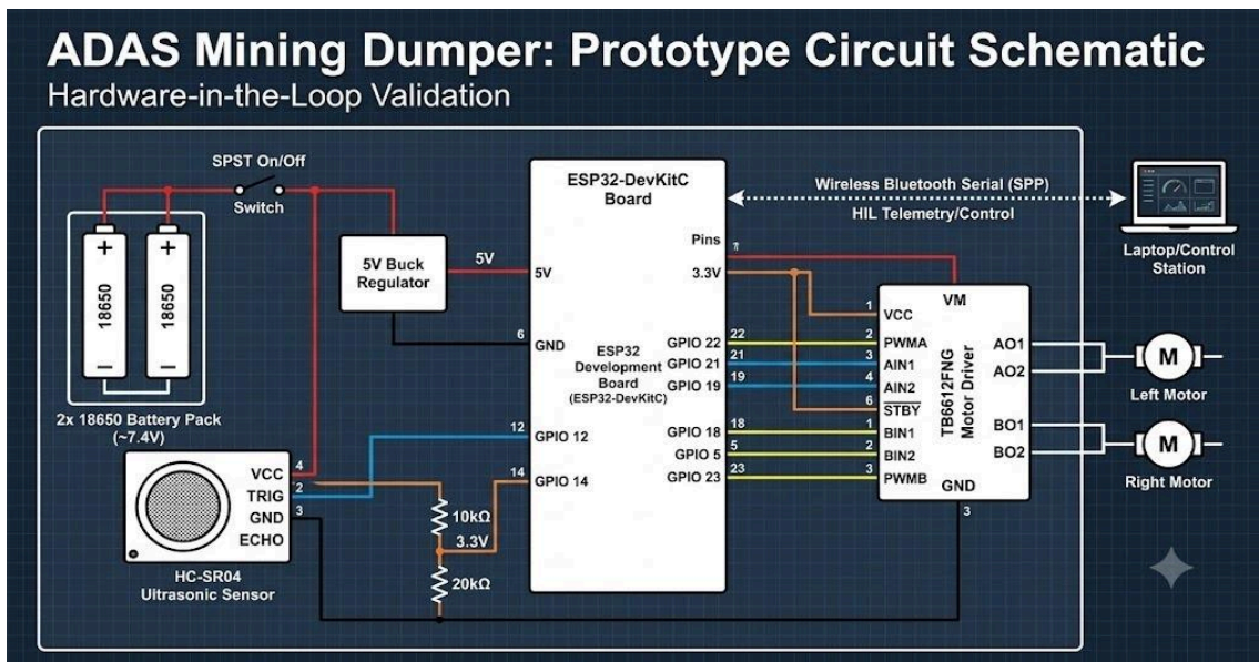
CIRCUIT DIAGRAM
